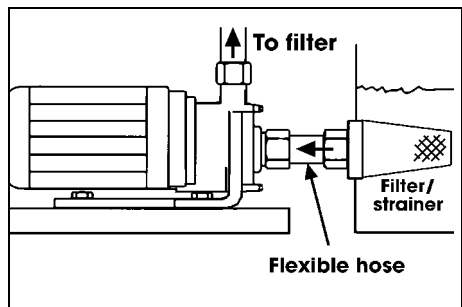
Fig 3: Gravity Feed
