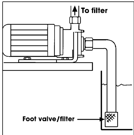
Fig 2:- Suction Lift
